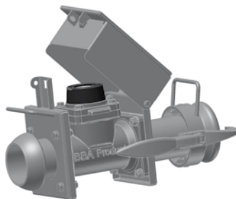
Siemens “Handy” flow meter, MAG 8000 battery powered, in portable casing
